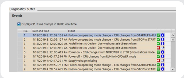
Fig. 2: PLC Diagnostic Buffer
